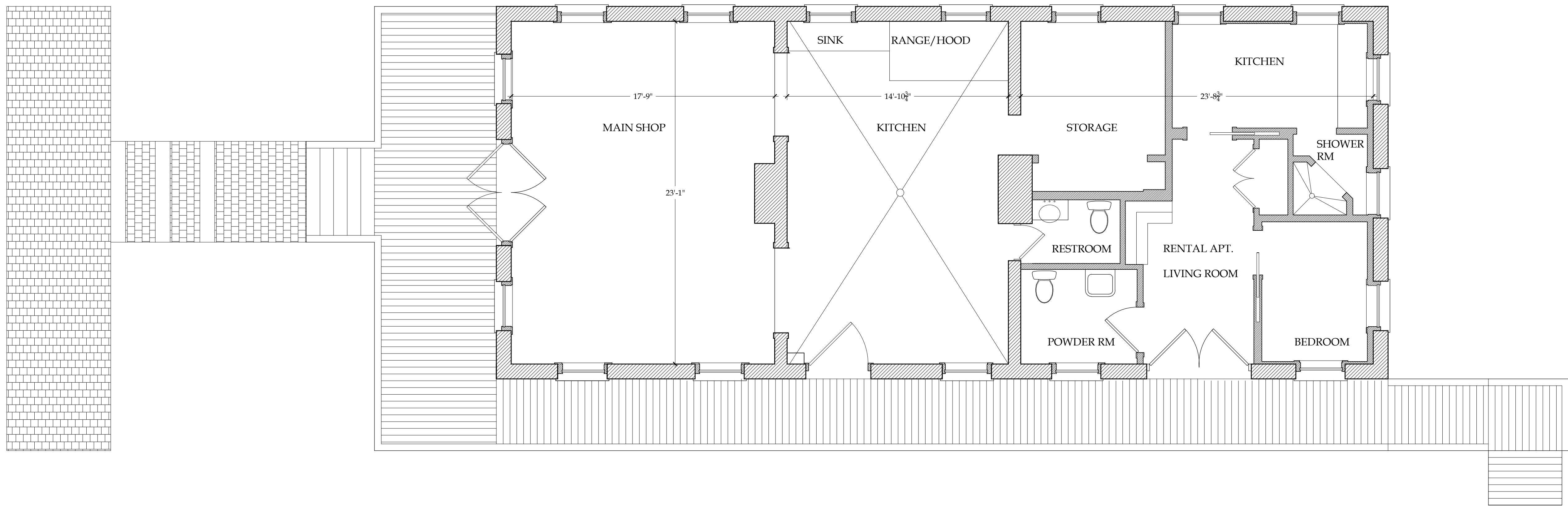
1 PLAN: EXISTING CONDITIONS EX-1.0 Scale: 1/4"=1'-0"
